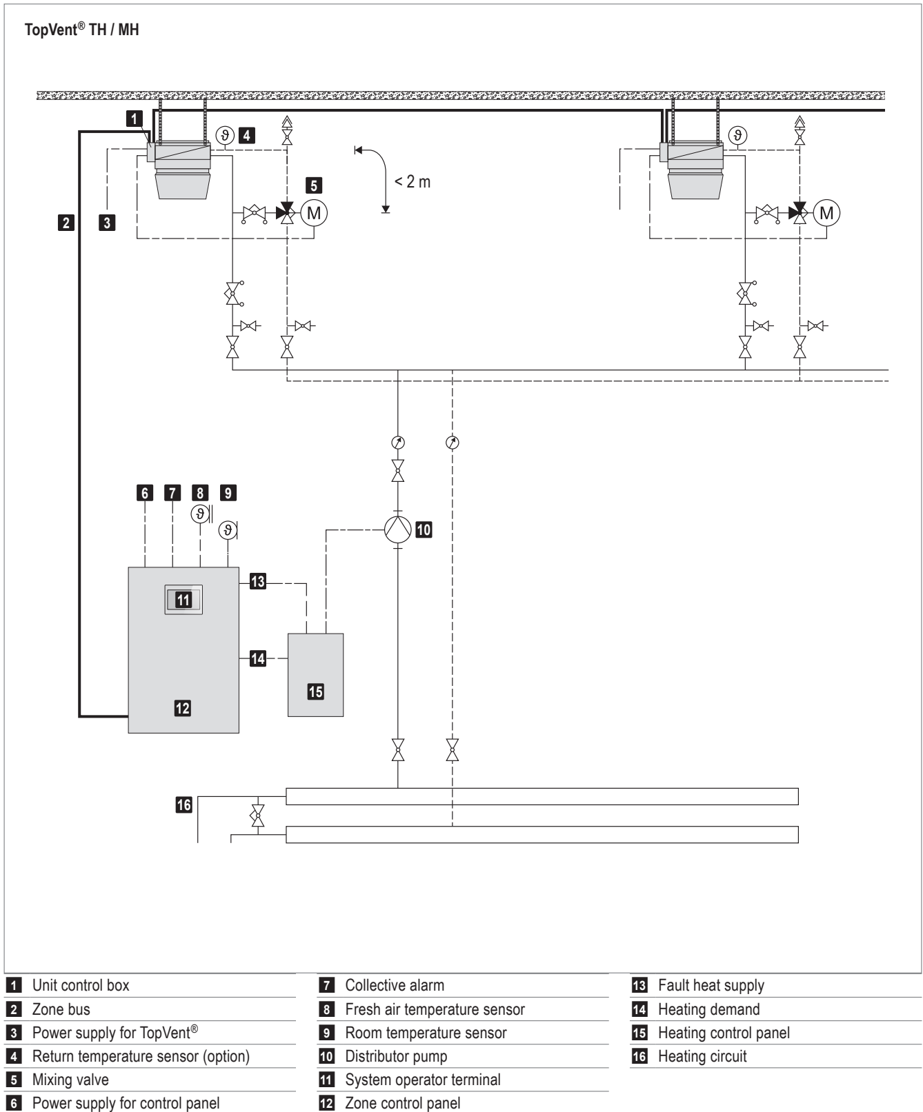
Fig. I2: Conceptual drawing for hydraulic diverting system TopVent® TH / MH
