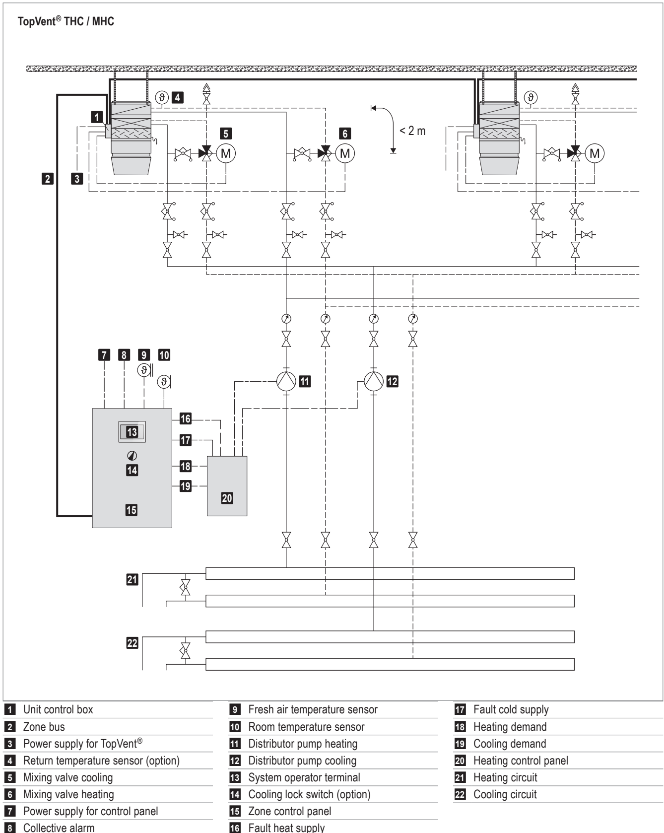
Fig. I4: Conceptual drawing for hydraulic diverting system TopVent® THC / MHC
