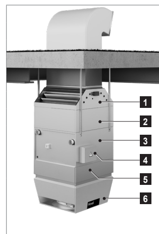
Fig. F1: TopVent® MC components
