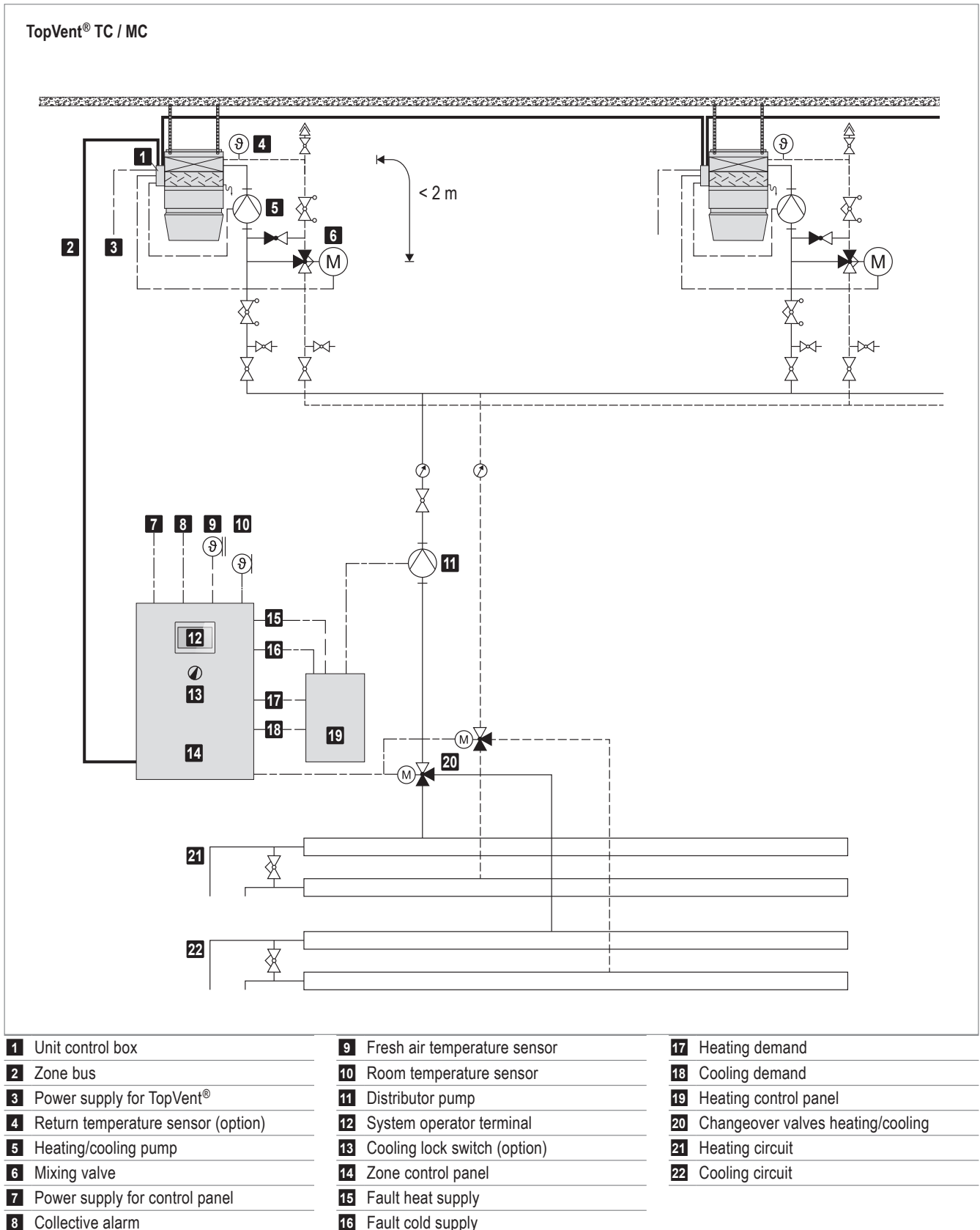
Fig. H7: Schematic diagram for injection system TopVent® TC / MC
