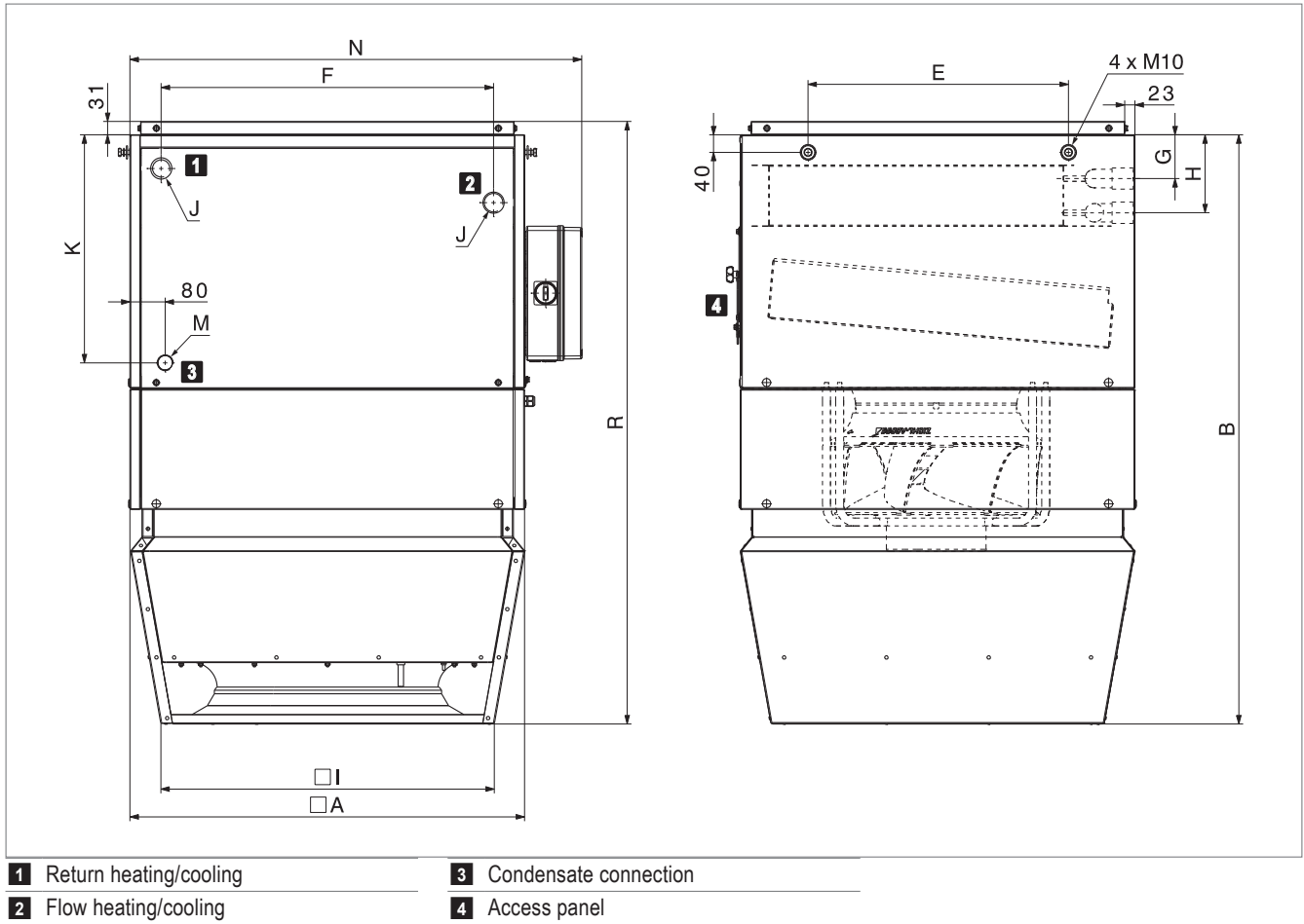
Fig. C4: TopVent® TC dimensional drawing
