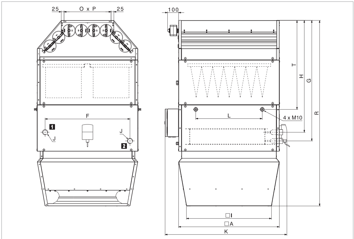
Fig. E4: TopVent® MH dimensional drawing
