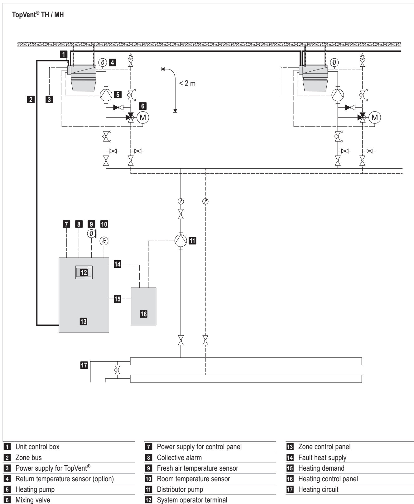
Fig. H6: Schematic diagram for injection system TopVent® TH / MH
