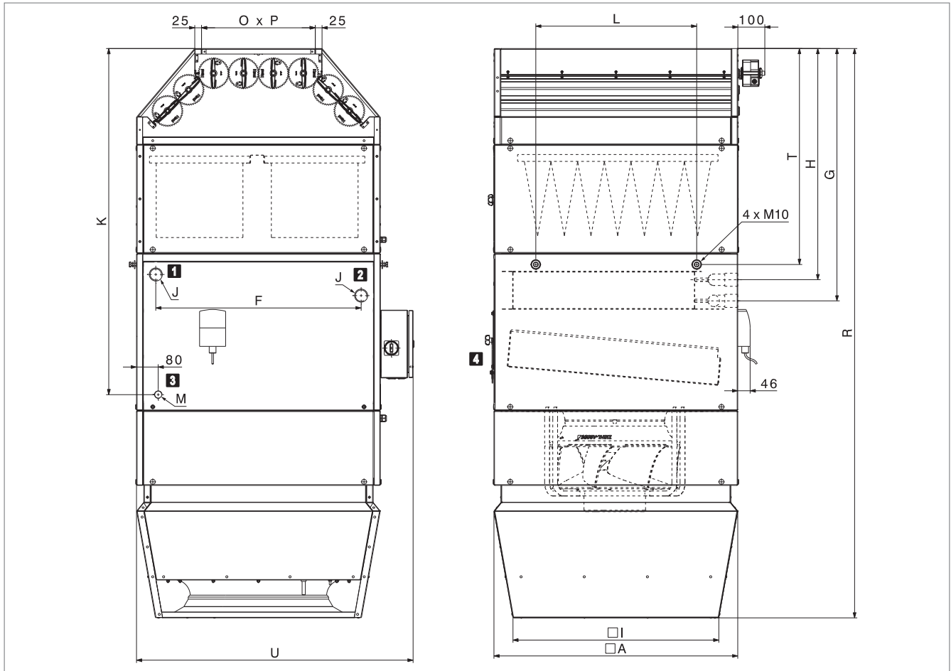
Fig. F4: TopVent® MC dimensional drawing
