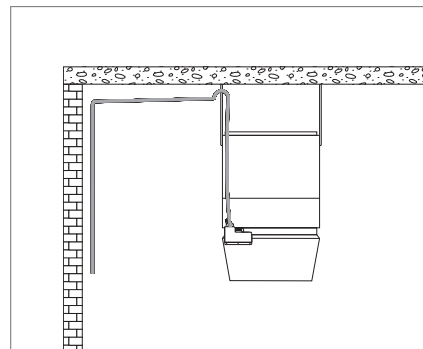
Fig. I1: Condensate drain
